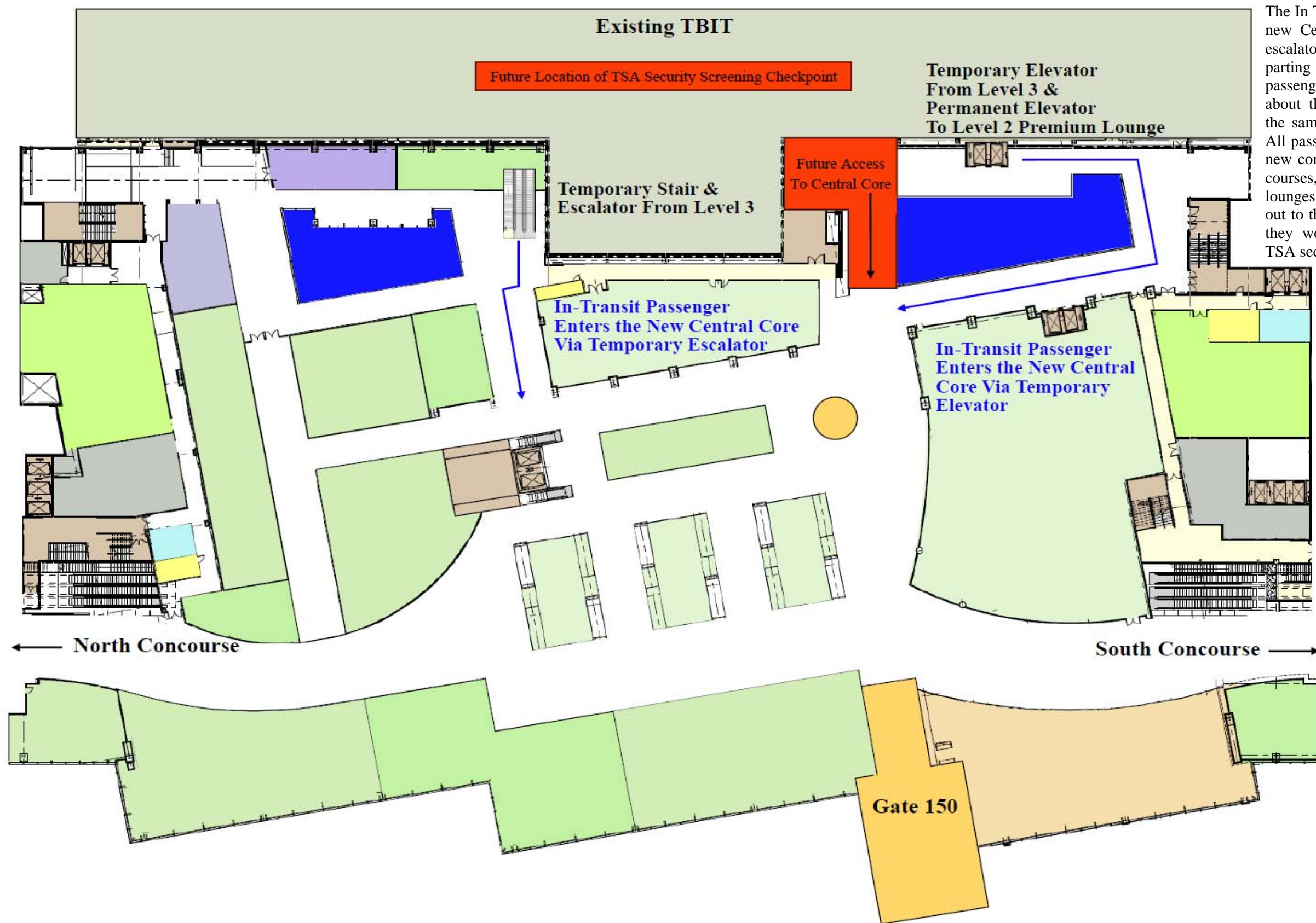
Level 4 - New Central Core/Departures Level
